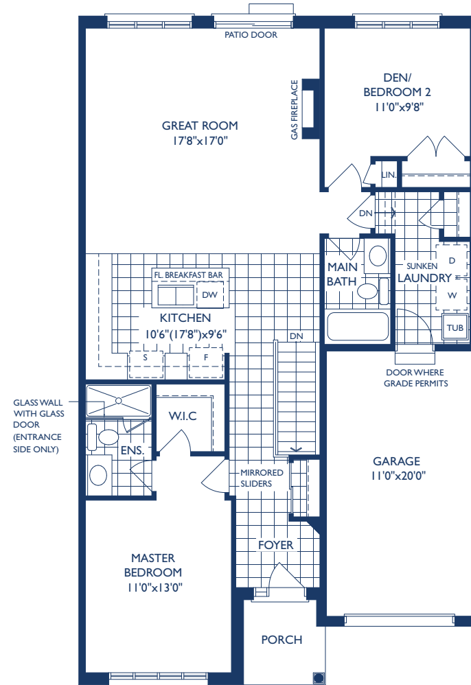
GROUND ELEV. A
